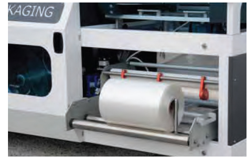
Film dispenser unit and film wind up unit both in front of the machine easy to be reached. Sliding door.
